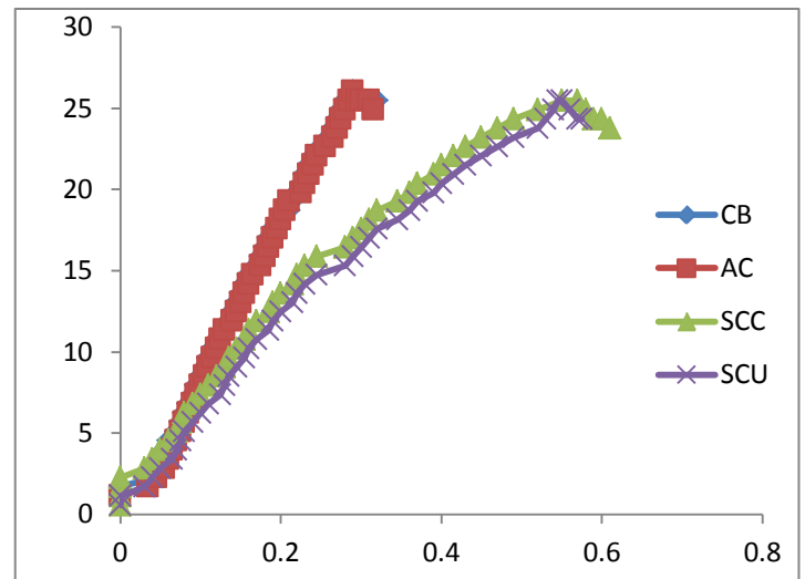
Fig 4. Load deflection behaviour under compression
